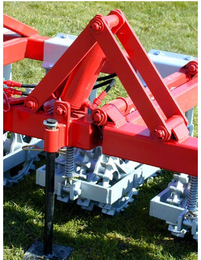
Repliage hydraulique
