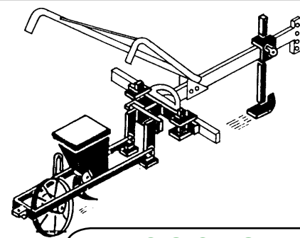
PRECISION SEEDER
